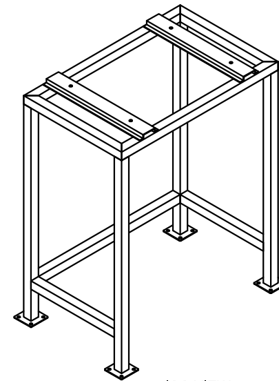
ISO VIEW
